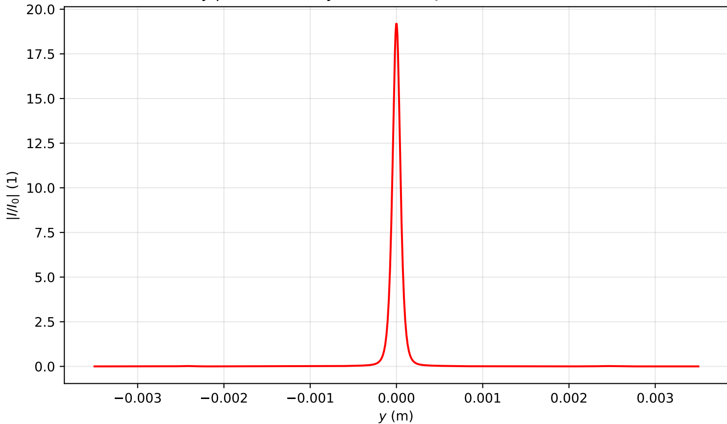
Intensity profile I(x = 0, y, z = 3.821)/I_0 , P_{in}=2.5P_{cr} , artificial time
